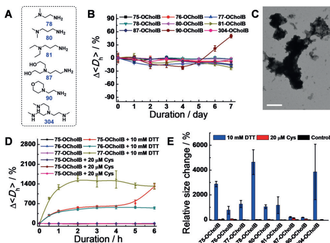
Figure 2. Stability test and reduction responsiveness study of OCholB LNPs. A) Chemical structures of amine heads. B) Relative hydrodynamic size variations of OCholB LNPs during storage. C) TEM image of 77-OCholB LNP after 10 mM DTT treatment. Scale bar = 600 nm. D) Time-dependent relative size variations of OCholB LNPs with DTT or Cys treatments. E) Relative size change of OCholB LNPs after 24 h of DTT or Cys incubation.
